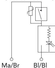
Circuito Reed NO
